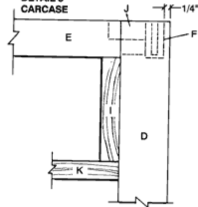
DETAIL 3 CARCASE
