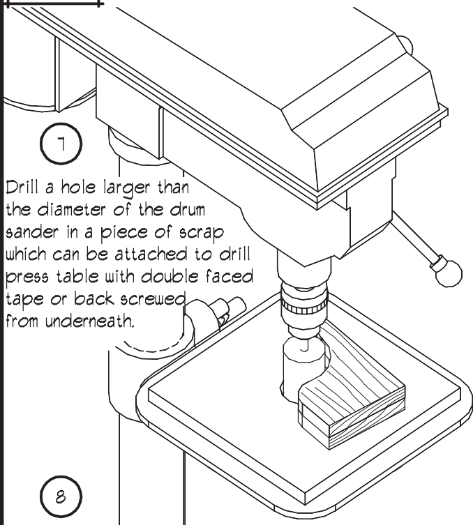
DIAG 6. SAND BRACKET CURVES
