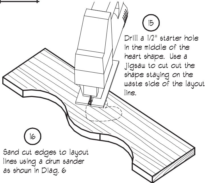
DIAG 12. CUT OUT HEART SHAPE
