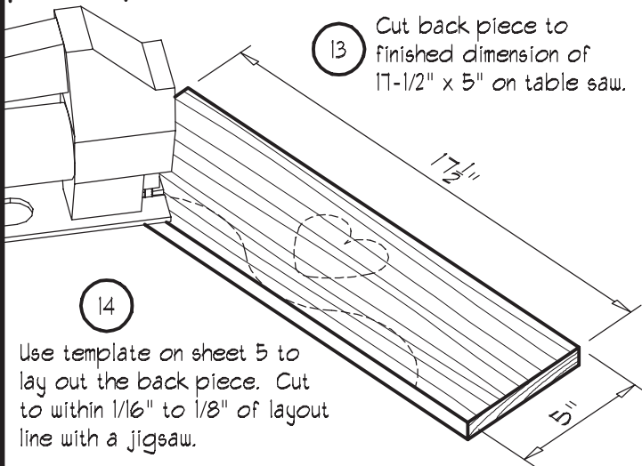
DIAG 11. CUT BACK PIECE (B.)
