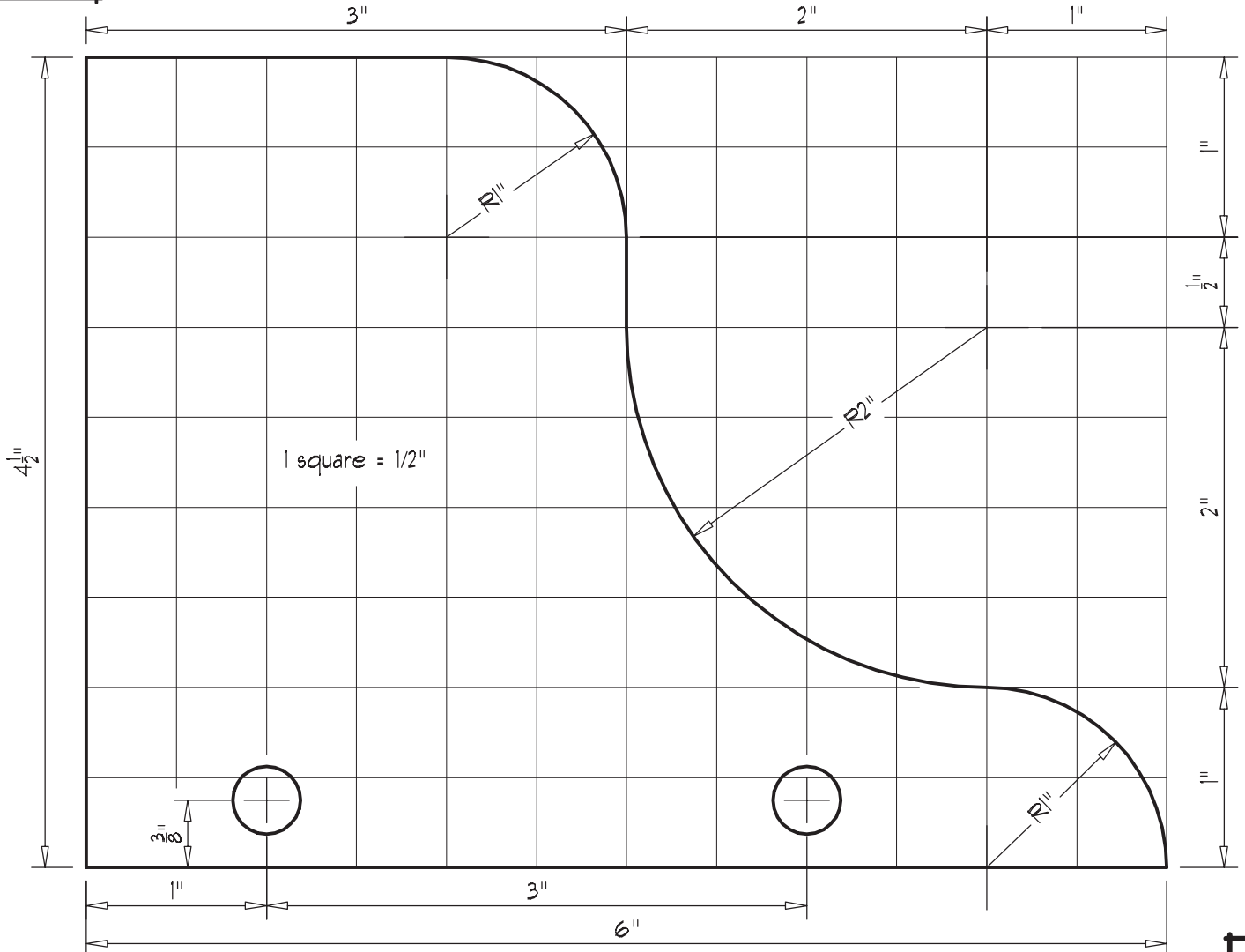
DIAG 5. BRACKET PATTERN
