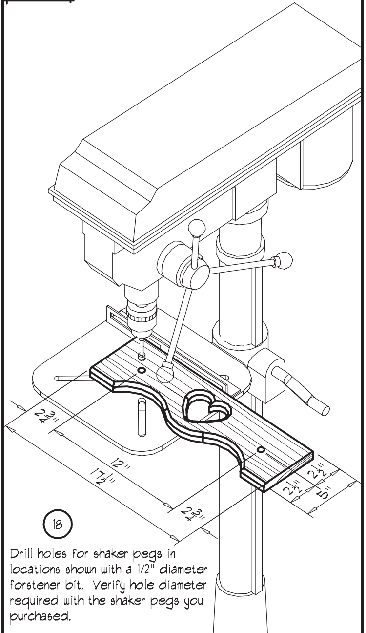
DIAG 14. DRILL HOLES FOR SHAKER PEGS
