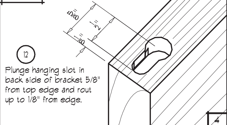
DIAG 10. HANGING SLOTS
